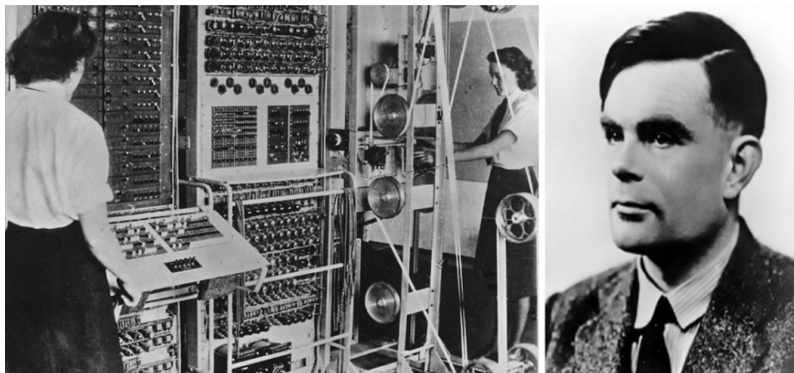
(foto: https://www.britannica.com/technology/computer/The-Turing-machine )
